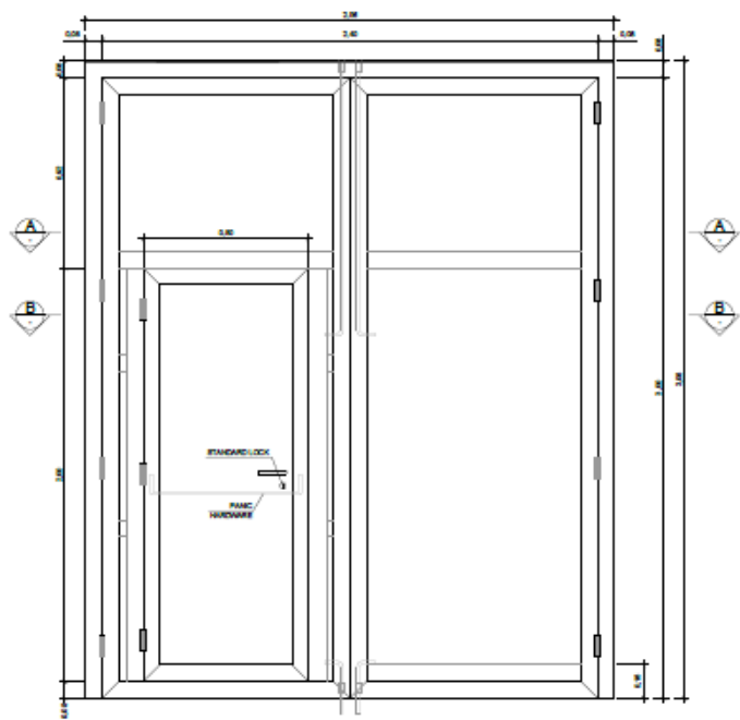
EXTERIOR ELEVATION DOOR (P1) scale 1:20
